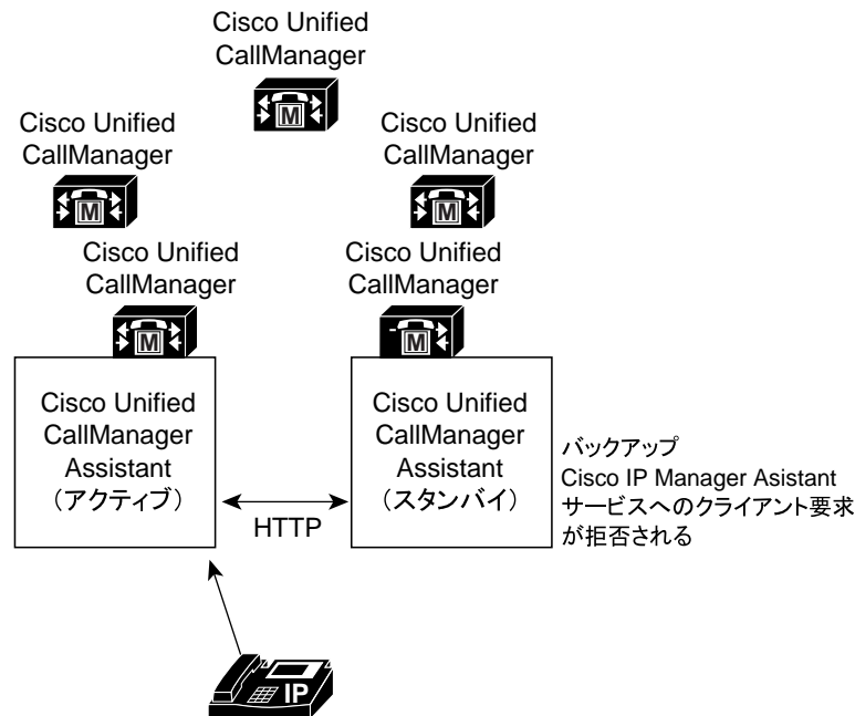
図 3-3 Cisco Unified CallManager Assistant の冗長化
