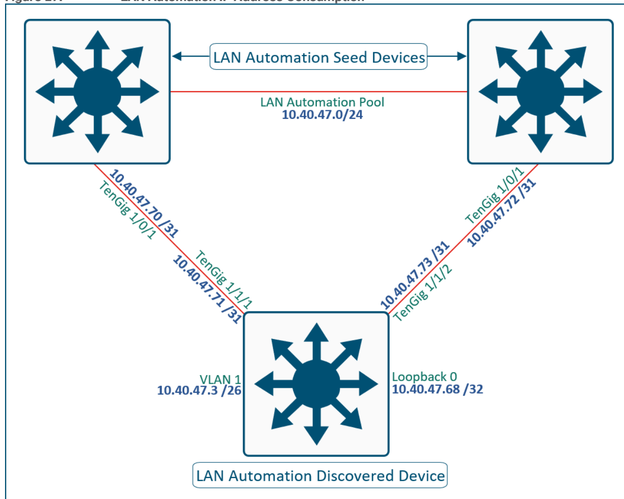
Figure 27. LAN Automation IP Address Consumption
