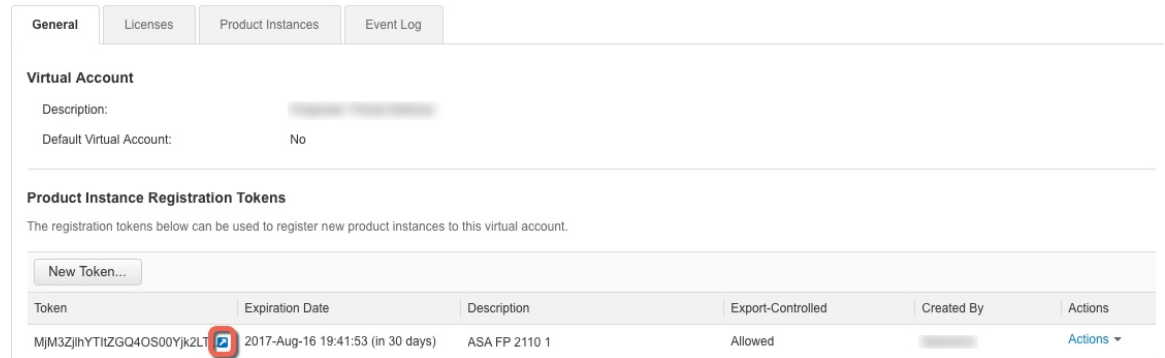
Figure 11: Copy Token
