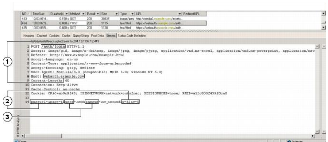
Figure 2: Action-uri, hidden, username and password parameters
