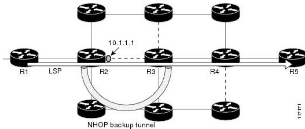
Figure 9: srlg exclude force--NHOP Autobackup Tunnel
