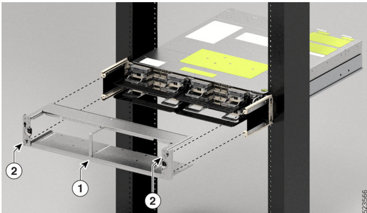
Figure 21: Installing the Air Filter Frame
