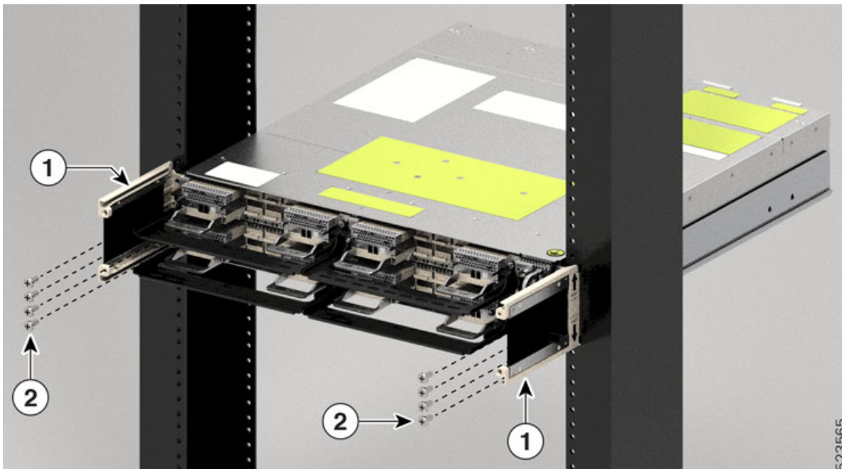
Figure 20: Installing the Air Filter Side Brackets
