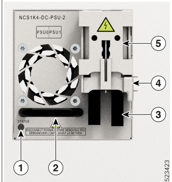
Figure 9: Front View of 2.5-kW DC PSU
