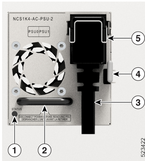
Figure 8: Front View of 2.5-kW AC PSU
