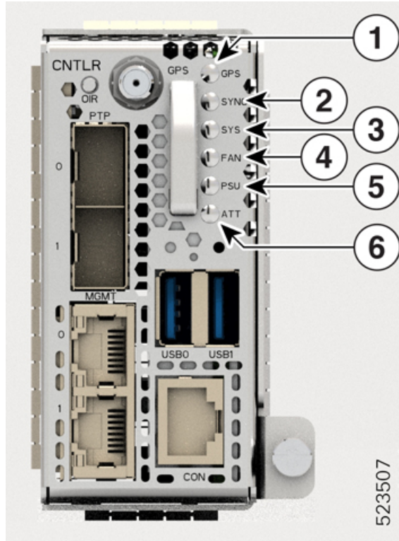
Figure 6: CNTLR LEDs
