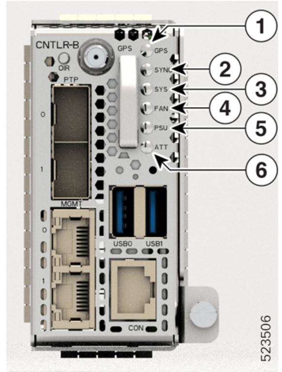
Figure 7: CNTLR-B LEDs
