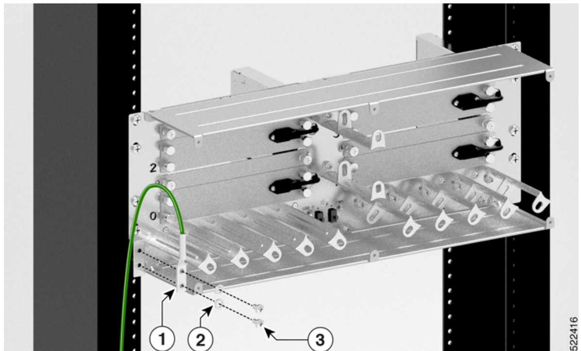
Figure 2: Front Side Grounding Option
