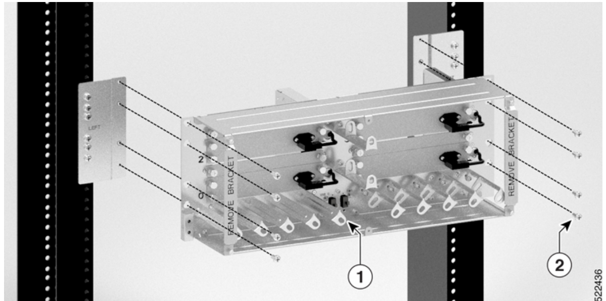
Figure 8: Installing Breakout Panel on a 23-inch Rack
