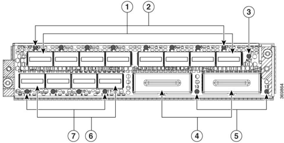
Figure 4: Front View of the OTN-XP Line Card
