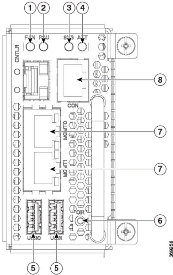
Figure 6: Front View of the Controller
