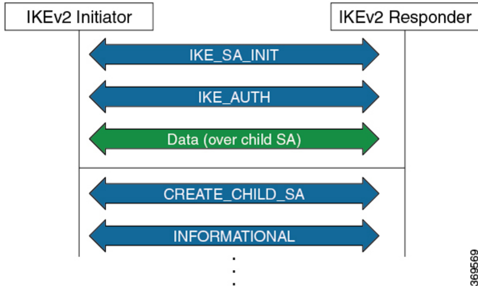
Figure 6: IKEv2 Exchanges
