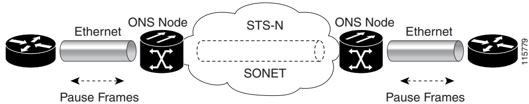
Figure 21-10 Flow Control
