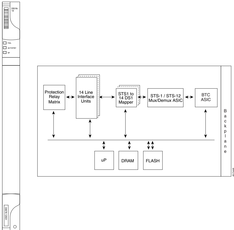
Figure 3-3 DS1N-14 Faceplate and Block Diagram
