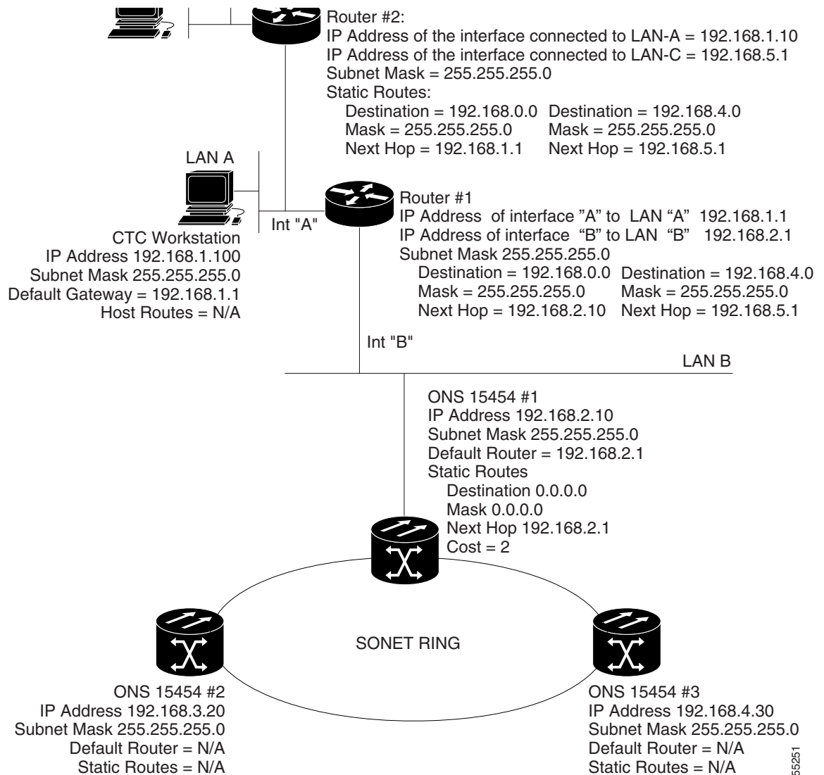
Figure 13-6 Scenario 5: Static Route With Multiple LAN Destinations
