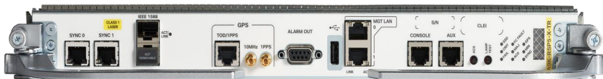
Figure 2. Cisco ASR 9000 Route Switch Processor RSP5-X - TR, Premium
