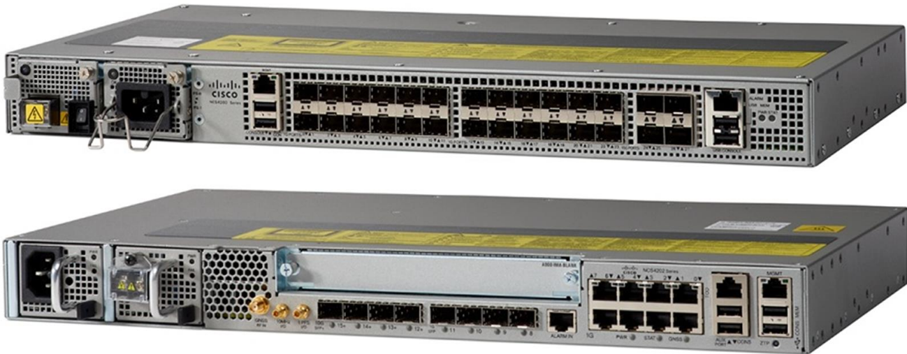
Figure 1. NCS 4201 and NCS 4202 Systems
