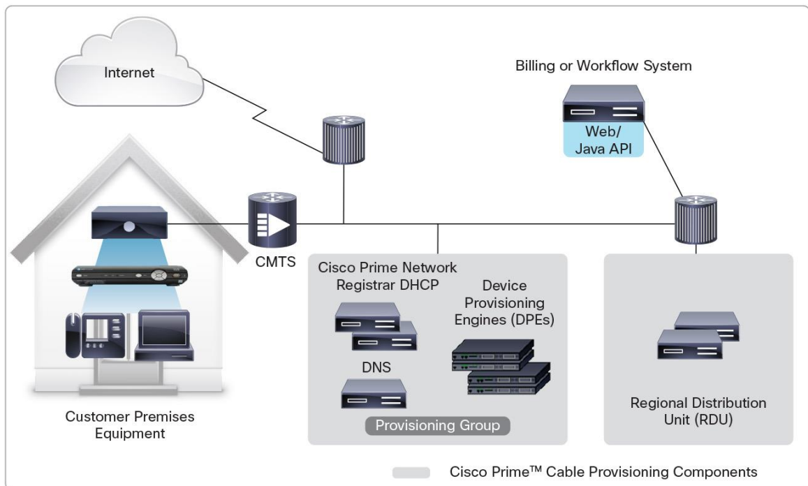
Figure 1. Cisco Prime Cable Provisioning Architecture
