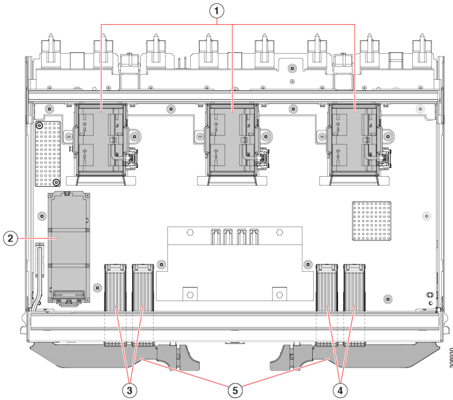
Figure 9 Cisco UCS 9108-100G IFM (top view)
