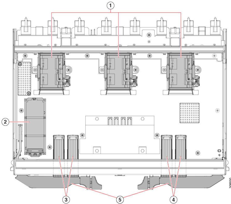
Figure 12 Cisco UCS Fabric Interconnect 9108 100G (top view)
