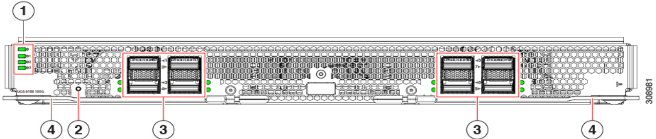
Figure 7 Cisco UCS 9108-100G IFM (front view)
