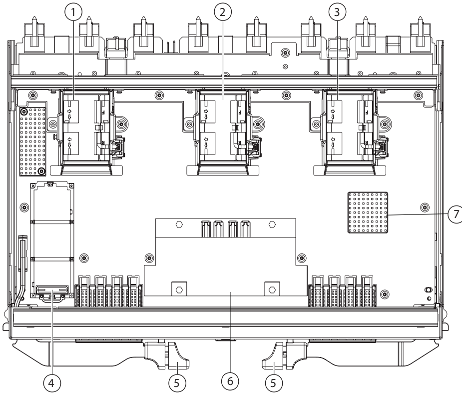
Figure 8 Cisco UCS 9108-25G IFM (top view)
