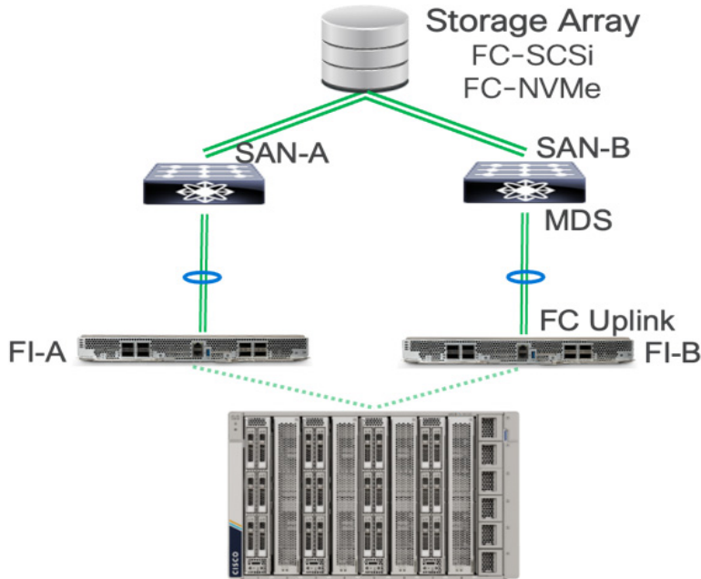
Figure 19 SAN Connectivity with Cisco UCS Fabric Interconnect 9108 100G and FC end-host or switch mode (Cisco MDS)
