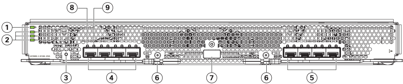
Figure 6 Cisco UCS 9108-25G IFM (front view)
