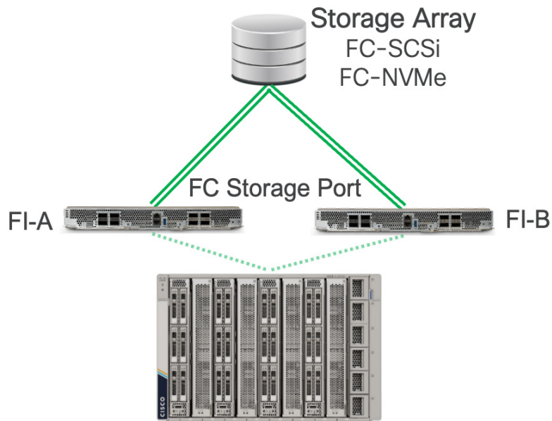
Figure 21 SAN Connectivity with Cisco UCS Fabric Interconnect 9108 100G and FC switch mode (direct attached)
