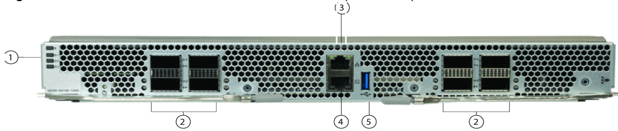
Figure 11 Cisco UCS Fabric Interconnect 9108 100G (front view)
