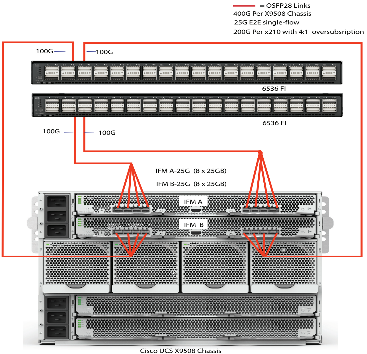
Figure 15 X9108-IFM-25G to 6536 Series Fabric Interconnects Connectivity
