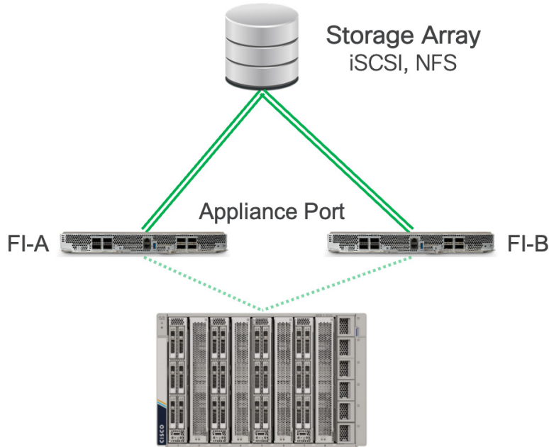
Figure 22 IP-SAN Connectivity with Cisco UCS Fabric Interconnect 9108 100G
