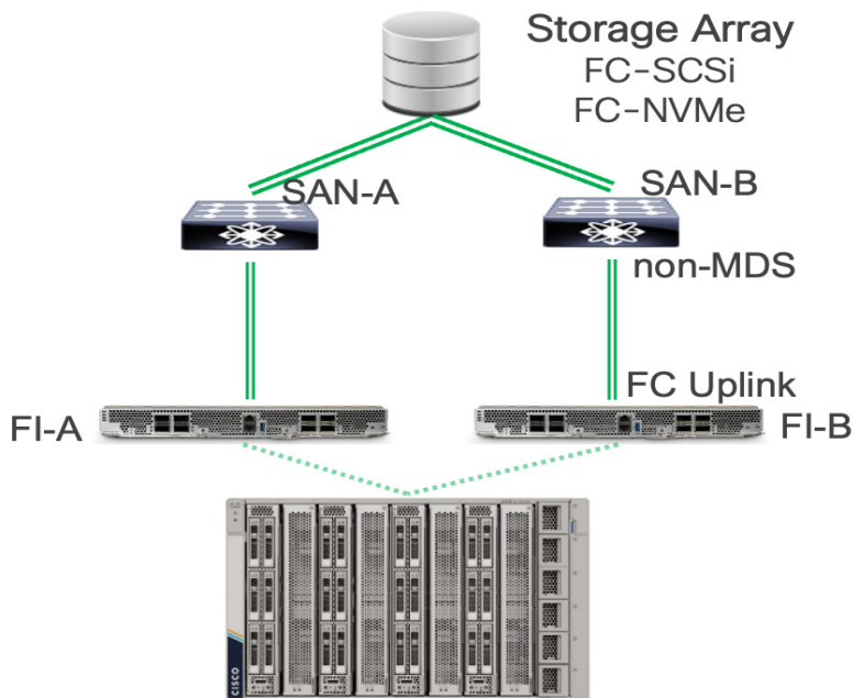
Figure 20 SAN Connectivity with Cisco UCS Fabric Interconnect 9108 100G and FC end-host mode (non-Cisco MDS)
