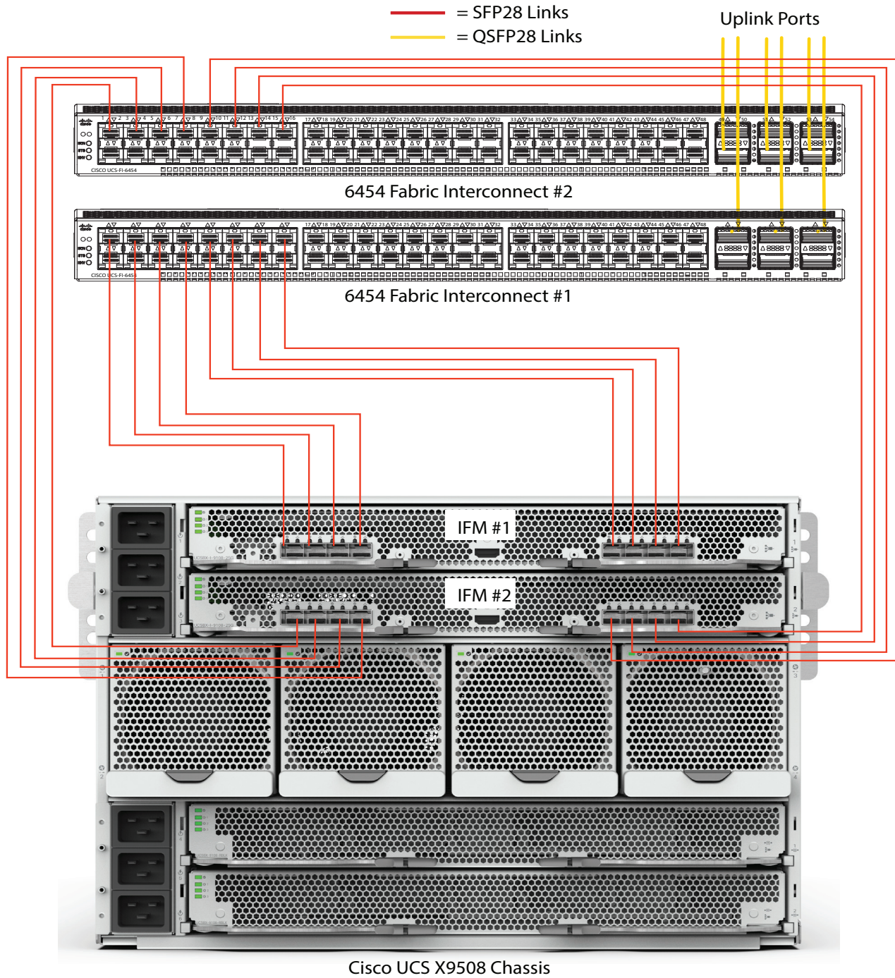
Figure 14 IFM to 6400 Series Fabric Interconnect Connectivity
