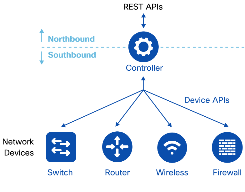
DIAGRAM Network Controller Architecture
