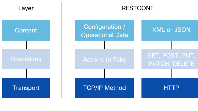
DIAGRAM RESTCONF Stack
