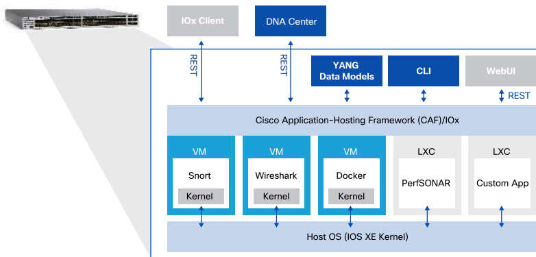
DIAGRAM Cisco Application Framework
