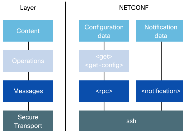
DIAGRAM NETCONF Stack
