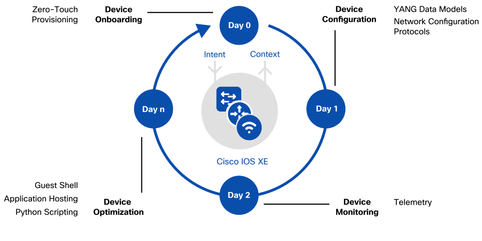
DIAGRAM Device Lifecycle Phases
